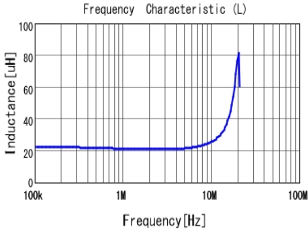
■ LQH44PH220MPR L
