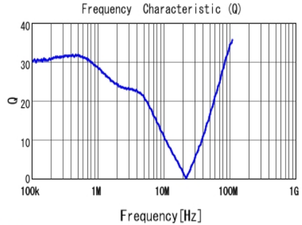
■ LQH44PH220MPR Q
