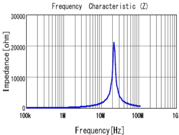
■ LQH44PH220MPR |Z|
