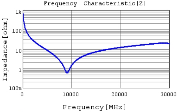
GRM0115C1E2R6WE01 |Z| DCOV,25degC
