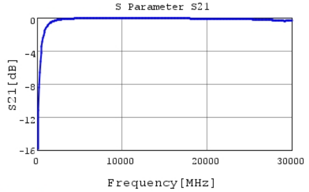
GRM0115C1E2R6WE01 S21 DCOV, 25degC
