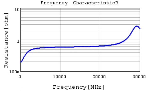
GRM0115C1E2R6WE01 R DCOV,25degC
