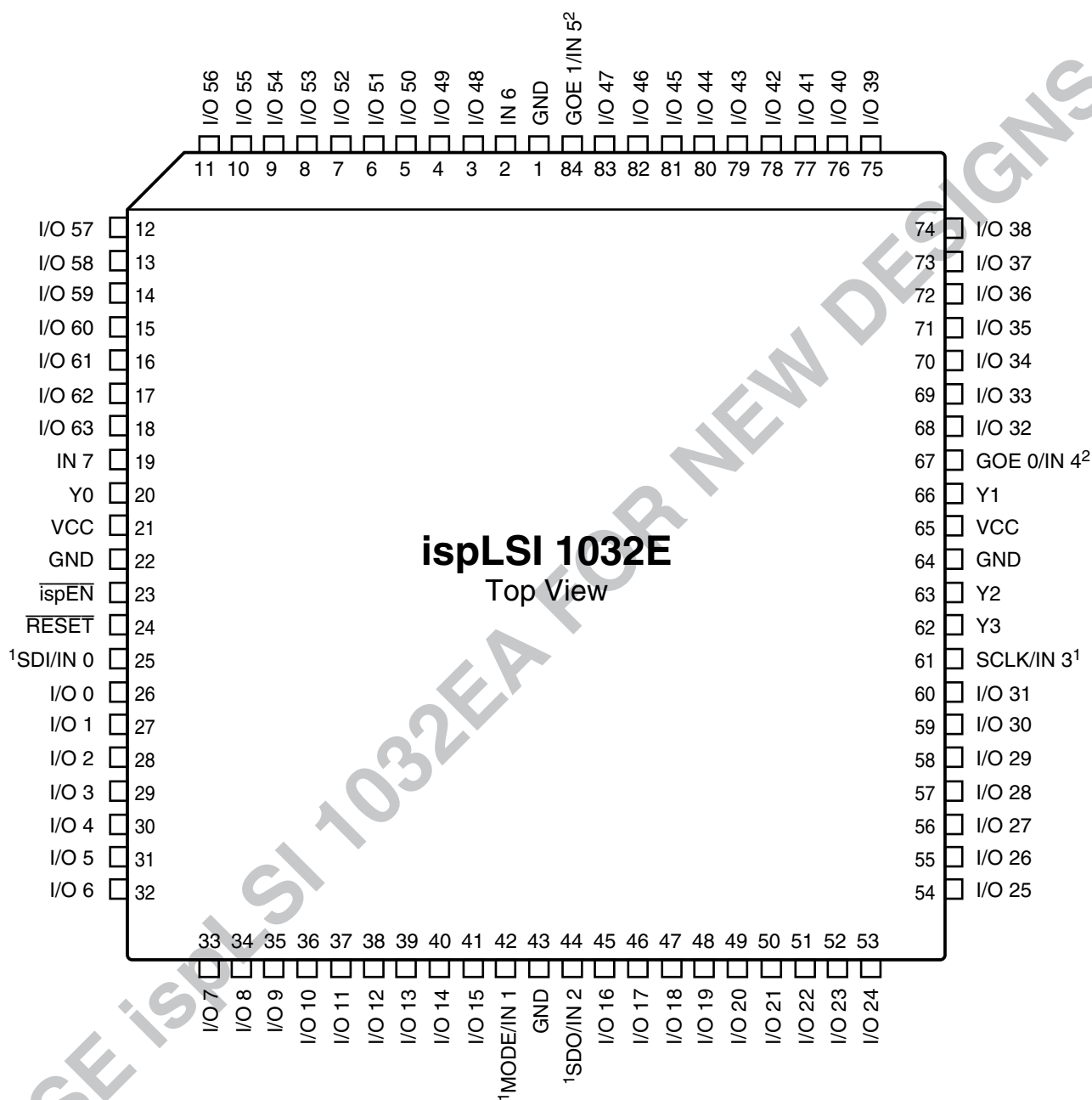
ispLSI 1032E 84-Pin PLCC Pinout Diagram
