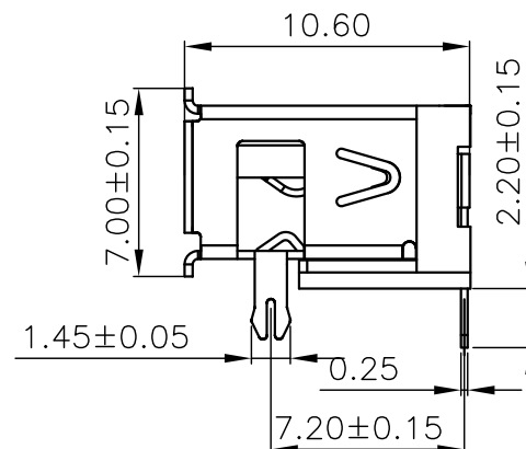
FRONT EDGE OF CONNECTOR PCB LAYOUT (T=1.60mm)
