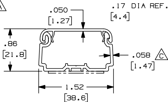
LDPH10 CLOSED POSITION
