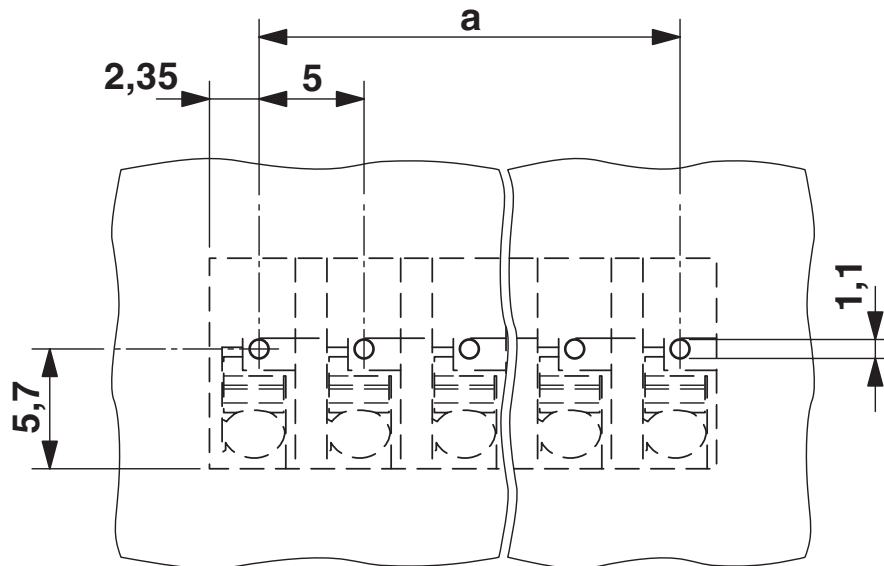
Dimensional drawing
