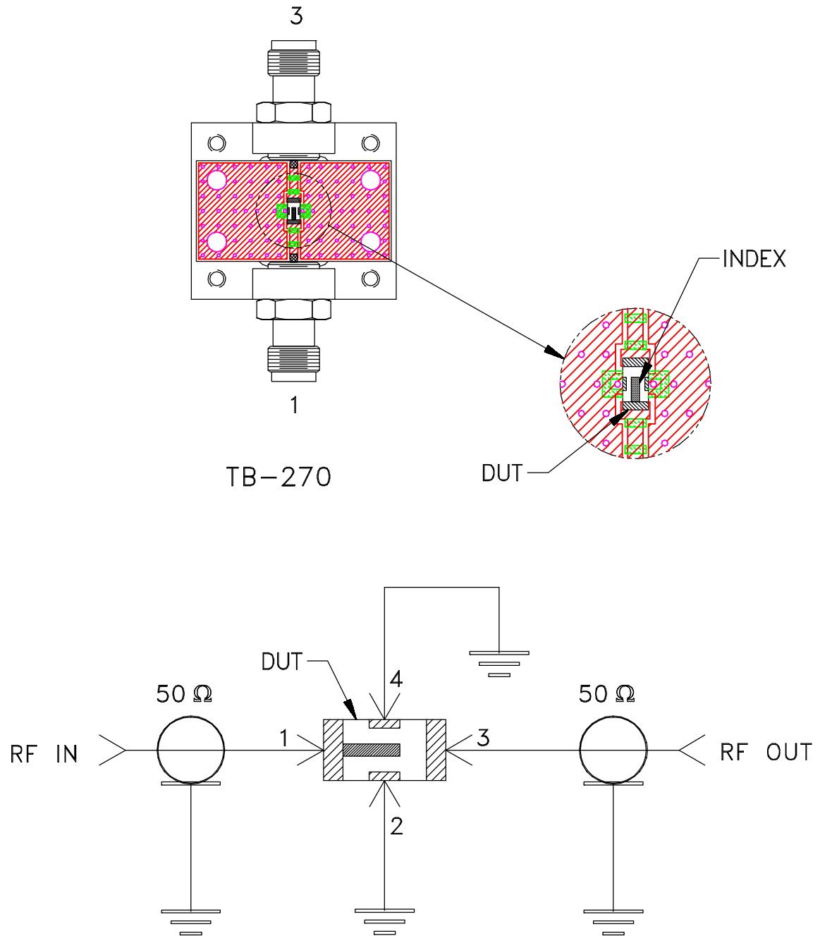
Schematic Diagram
