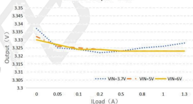
Load VS Output—3.3V
