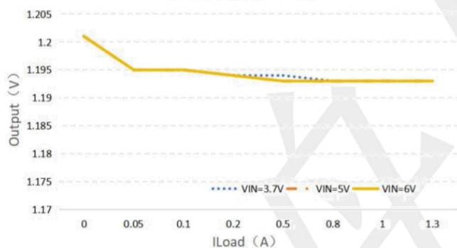
Load VS Output—1.2V
