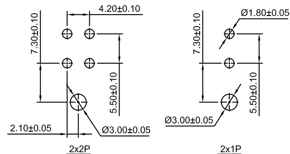
P.C.B LAYOUT Recommended PCB Thickness 1.78MAX
