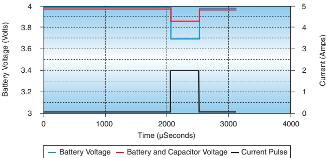
Figure 5. GSM Pulse
