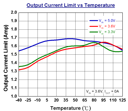
Figure 15. Output Current Limit vs. Temperature
