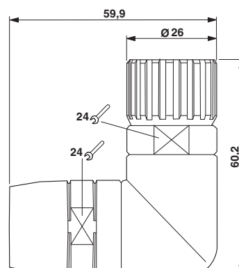
Dimensional drawing
