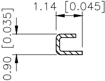
SECTION:C-C SCALE:1:1
