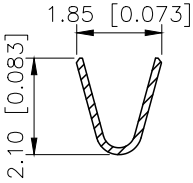
SECTION:A-A SCALE:1:1
