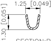
SECTION:B-B SCALE:1:1
