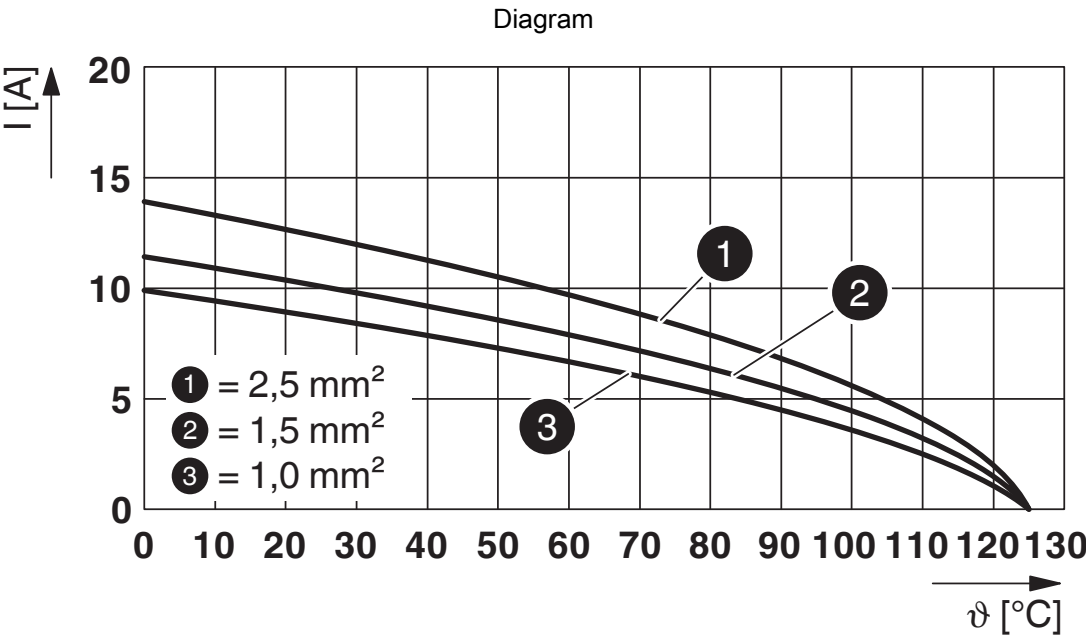
Derating diagram rolled contacts
