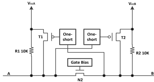
Architecture of TXS0104EPWR
