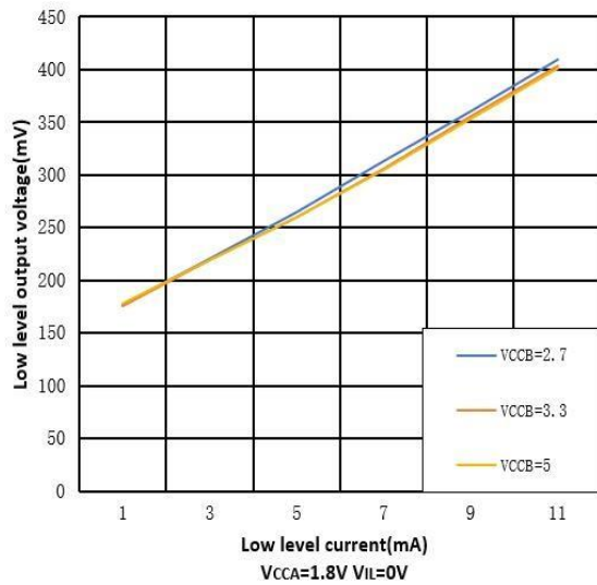
Low Level Output Voltage vs Low Level Current
