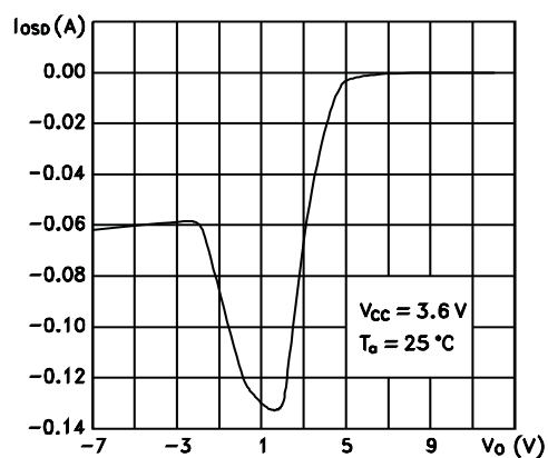
Driver short-circuit current
