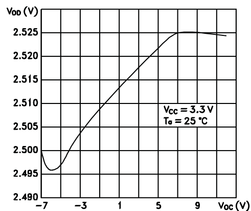
High level driver output capability
