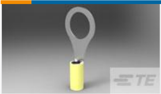
TE Part #160138 PIDG RING TONGUE
