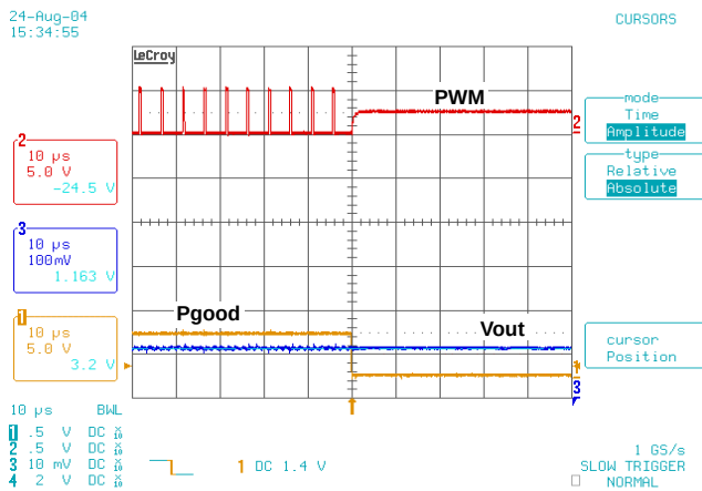
FIGURE 27. UNDERVOLTAGE RESPONSE SHOWING PWM TRI-STATE, VOUT &lt; VID - 300mV
