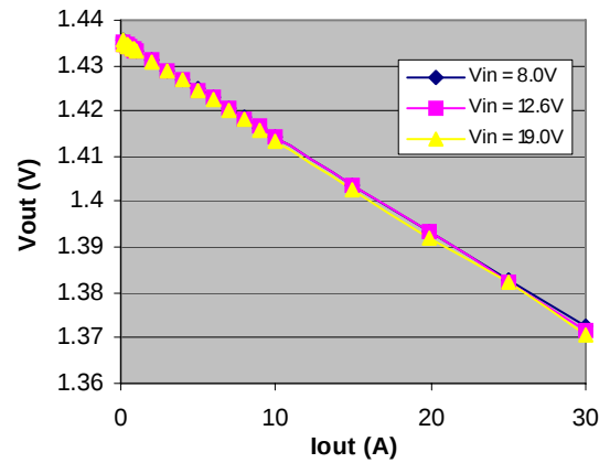
FIGURE 4. DEEPER SLEEP MODE LOAD LINE, 3 PHASE, CCM, PSI# = LOW VID= 1.435V
