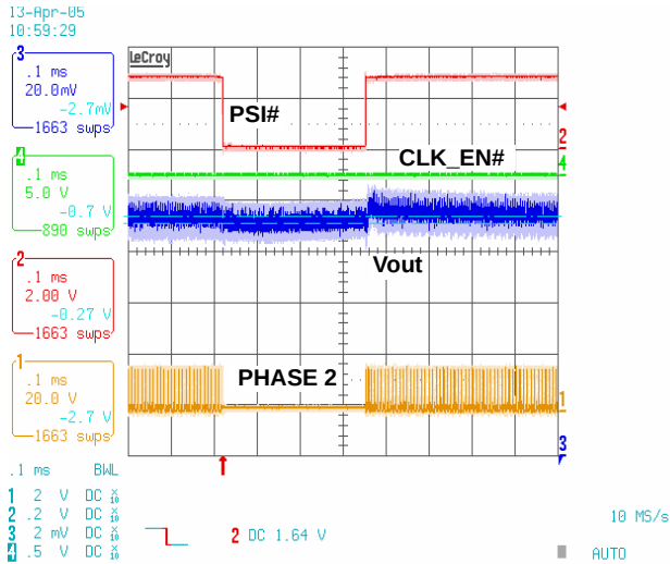
FIGURE 31. ISL6260B PHASE ADDING AND DROPPING IN DEEPER SLEEP MODE, LOAD CURRENT = 4.35A
