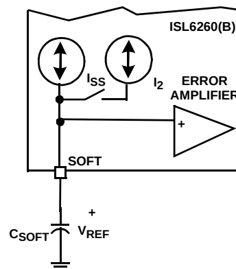
FIGURE 40. SOFT PIN CURRENT SOURCES FOR FAST AND SLOW SLEW RATES
