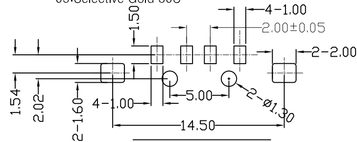
FRONT EDGE OF CONNECTOR PCB LAYOUT
