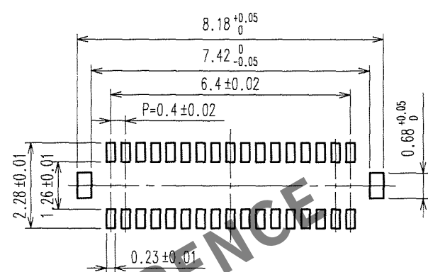
RECOMMENDED METAL MASK OPENING PATTERN
