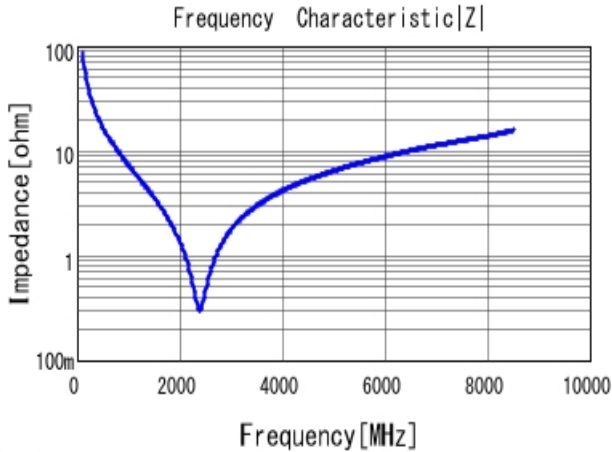
■ GRM0332C1H180GA01 |Z| DC0V, 20degC
