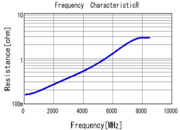
■ GRM0332C1H180GA01 R DC0V, 20degC
