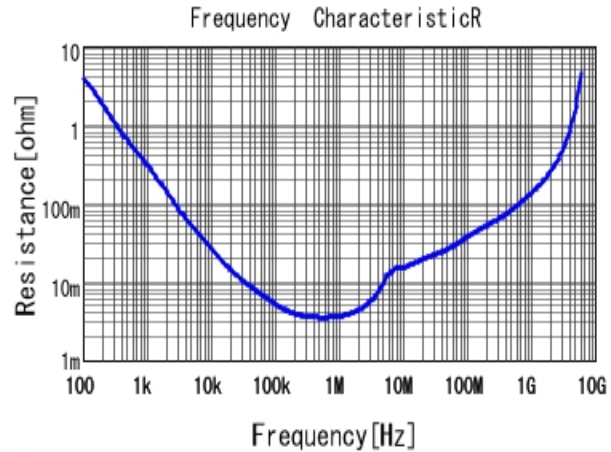
■ GRM188R61A475MAAJ R DC0V, 25degC
