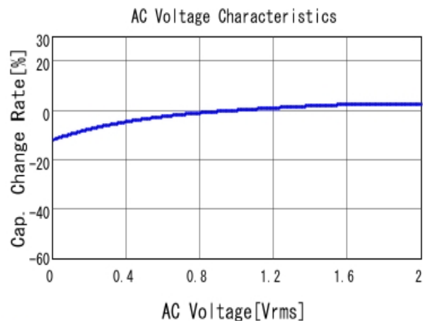
■ GRM188R61A475MAAJ C-AC Voltage capchange, DC0V, 25.0d
