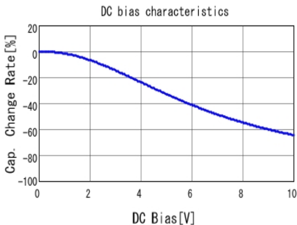
■ GRM188R61A475MAAJ C-DC bias capchange, 25.0degC, AC1.
