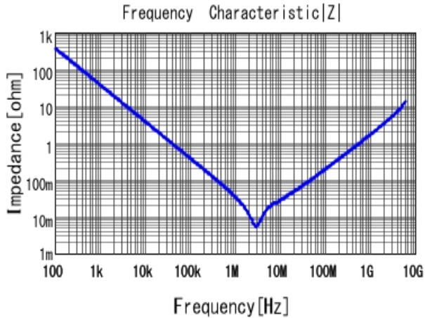
■ GRM188R61A475MAAJ |Z| DC0V, 25degC
