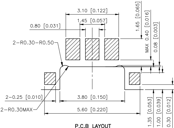
P.C.B LAYOUT VIEW FORM THE DIRECTION A
