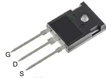
TO247 (TO-247-3)
