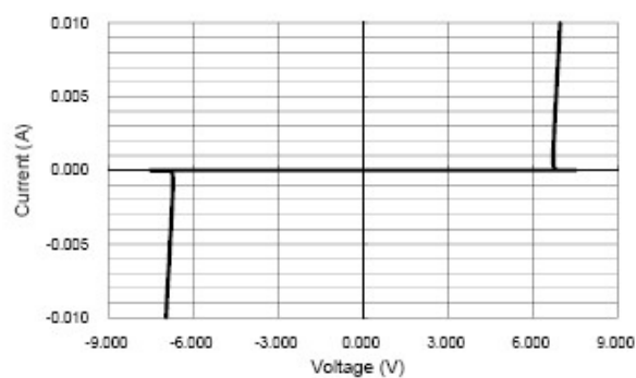
Fig 3 Voltage Sweeping
