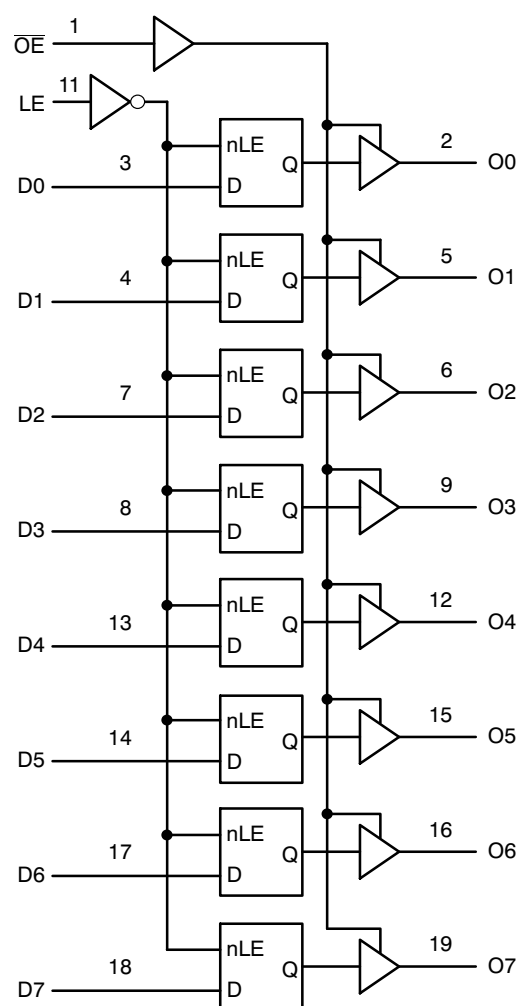
Figure 2. Logic Diagram
