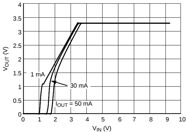
Figure 7. Output Voltage vs. Input Voltage 3.3 V Version
