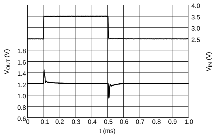
Figure 24. Line Transients, 1.2 V Version, I_{OUT} = 1 mA
