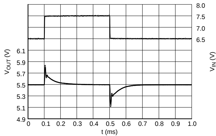
Figure 26. Line Transients, 5.5 V Version, I_{OUT} = 1 \text{ mA}
