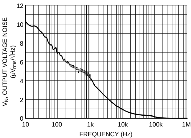
Figure 19. Output Voltage Noise, 3.3 V Version, V_{IN} = 4.3\text{ V} , I_{OUT} = 30\text{ mA} , C_{in} = C_{out} = 0.1\text{ }\mu\text{F}
