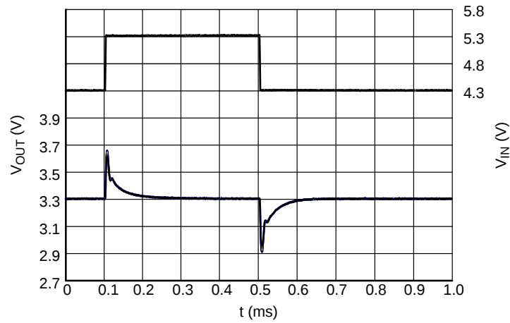
Figure 25. Line Transients, 3.3 V Version, I_{OUT} = 1 \text{ mA}
