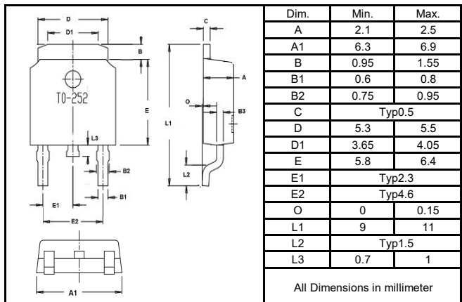
T0-252
