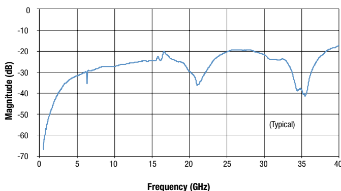
ATC 560L Series Return Loss (S11)
