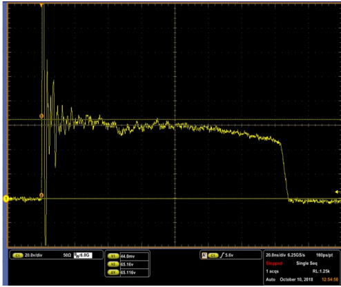
AQHV36-C +8kV Contact ESD Clamping Voltage
