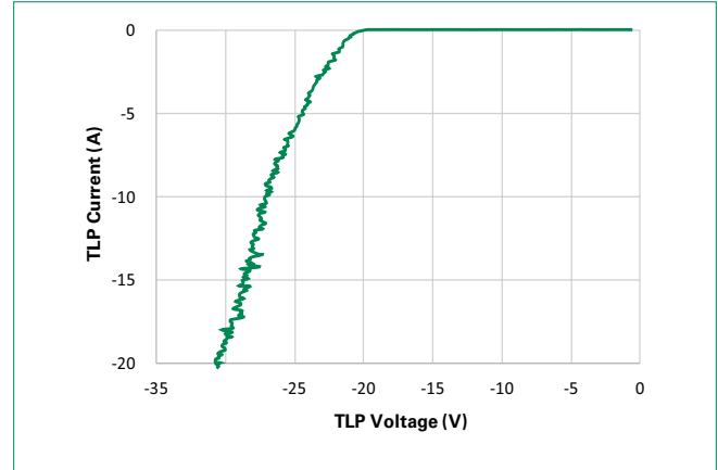
AQHV15-C Negative Transmission Line Pulsing(TLP) Plot
