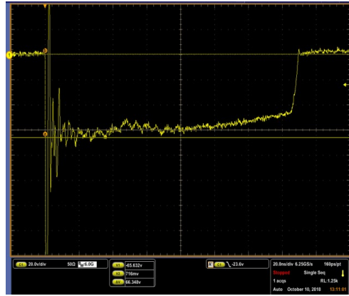
AQHV36-C -8kV Contact ESD Clamping Voltage
