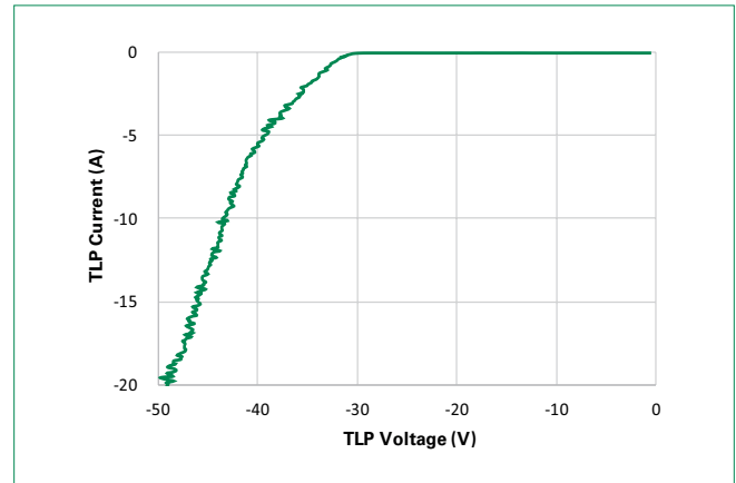
AQHV24-C Negative Transmission Line Pulsing(TLP) Plot
