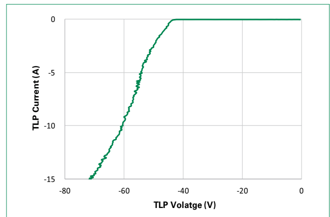
AQHV36-C Negative Transmission Line Pulsing(TLP) Plot
