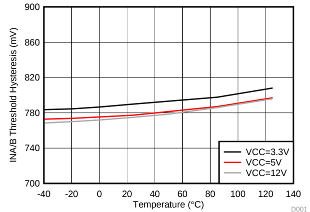
Figure 19. INA/B Hysteresis vs. Temperature
