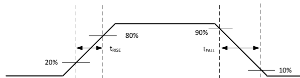
Figure 28. Rising and Falling Time Criteria
