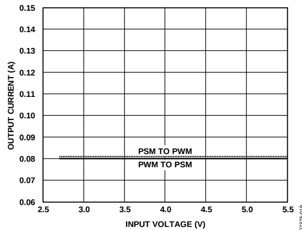
Figure 9. Mode Transition
