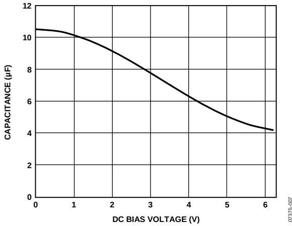
Figure 30. Typical Capacitor Performance
