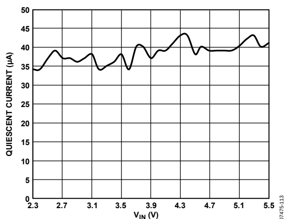
Figure 14. Quiescent Current vs. Input Voltage ( V_{OUT} = 3.3 V)
