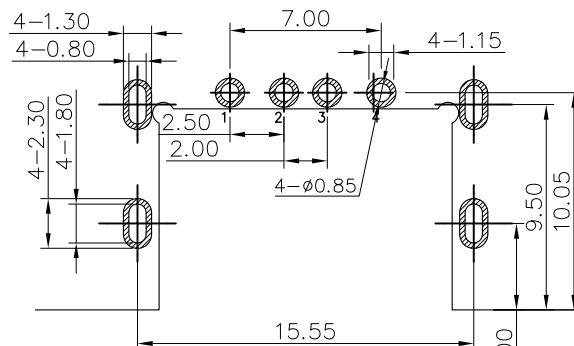
RECOMMENDED P.C.B HOLE LAYOUT COMPONENT SIDE VIEW(TOLERANCE: \pm 0.05 )
