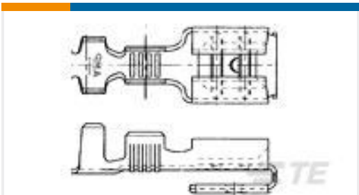
TE Part #160739-2 250 FASTON,PIGGYBACK REC.,18-14 AWG,TPBR
