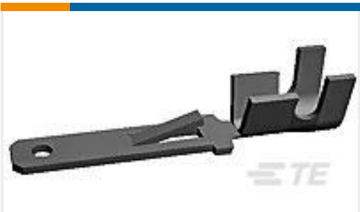
TE Part #928947-2 FF 250 TAB 17-13 AWG .016 TPBR
