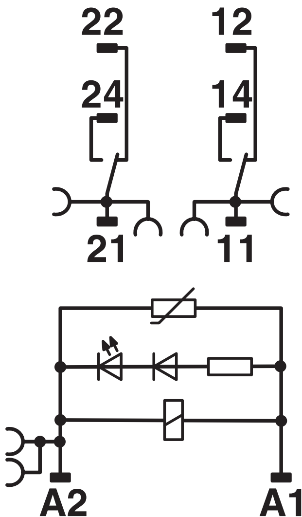
Circuit diagram
