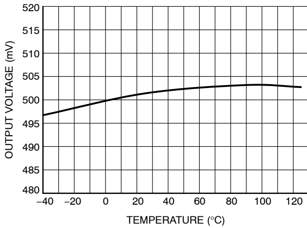
Figure 9. Output Voltage vs. Temperature
