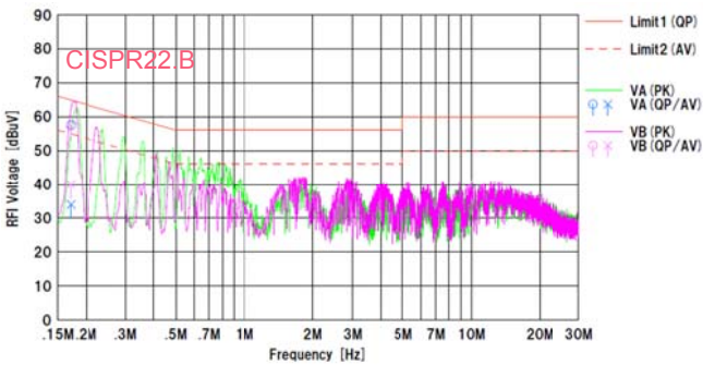
Figure 22. Conducted Emission.2
