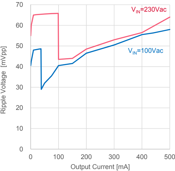
Figure 14. VOUT Ripple Voltage ( I_{OUT} vs. V_{ripple} )
