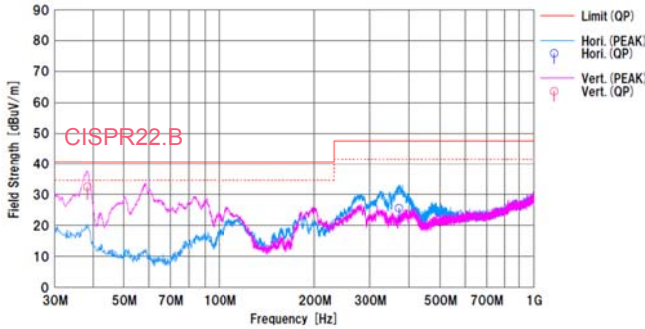
Figure 24. Radiated Emission.2
