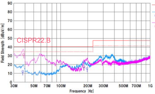
Figure 23. Radiated Emission.1
