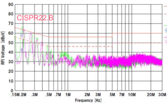
Figure 21. Conducted Emission.1
