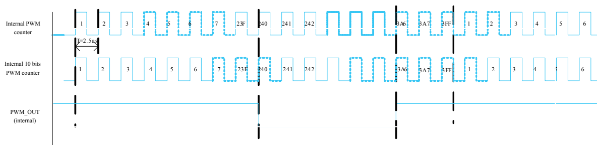
Figure 16. Resulting waveform 4
