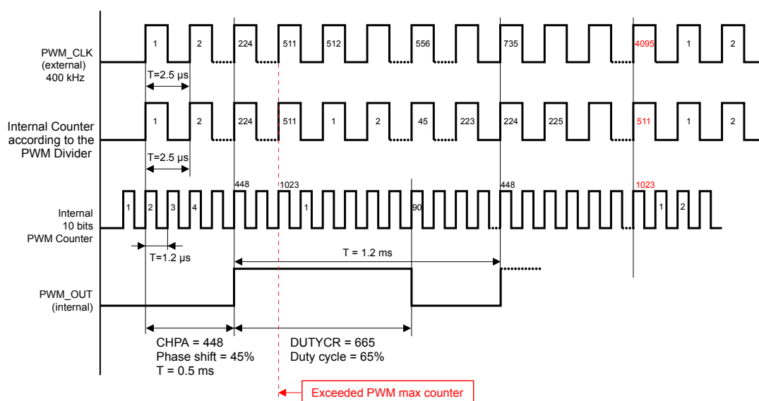
Figure 15. Resulting waveform 3
