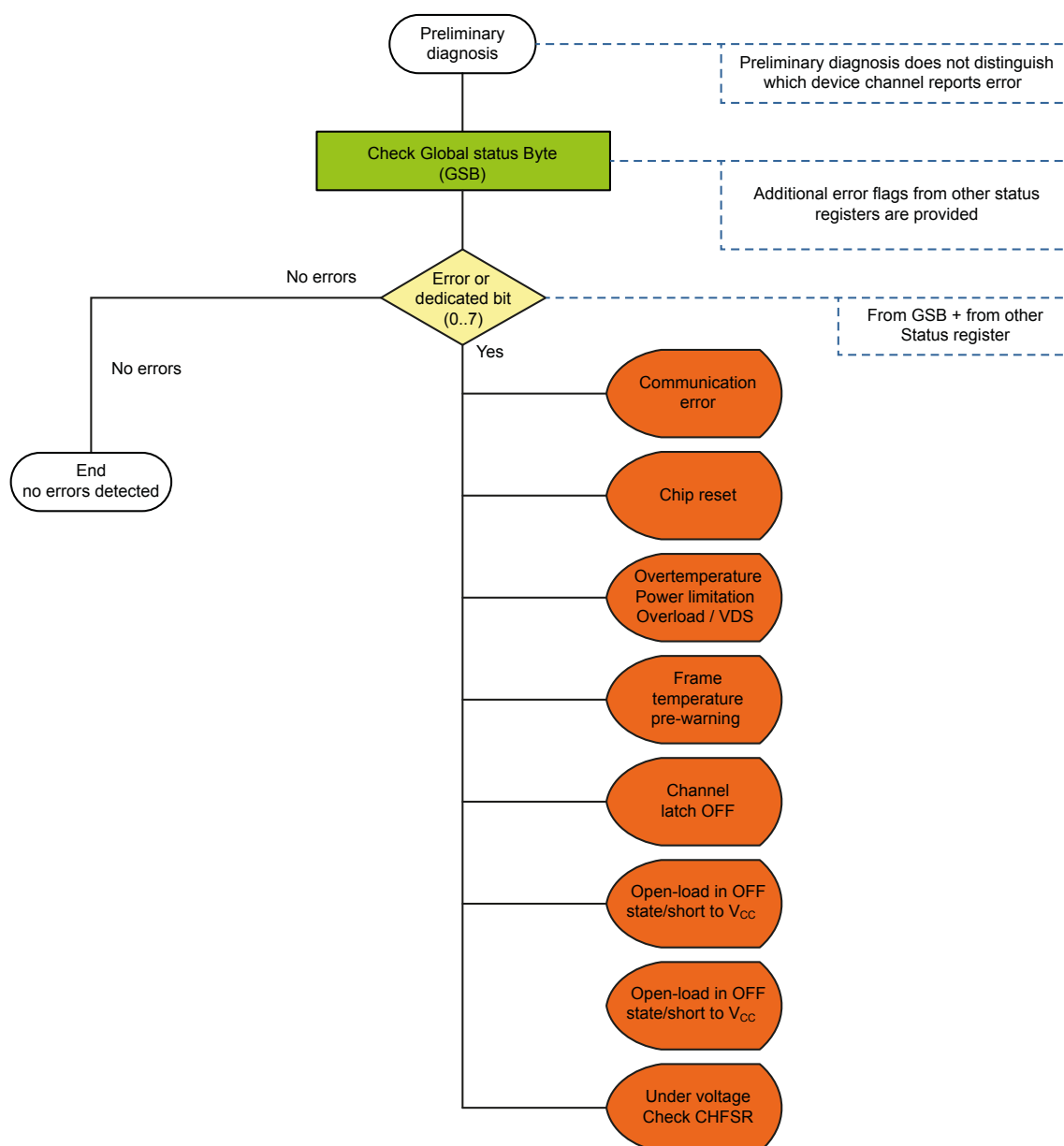
Figure 24. Status registers
