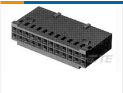
TE Part #2-87631-1 26 MODIV HSG COMP DR .100 POL
