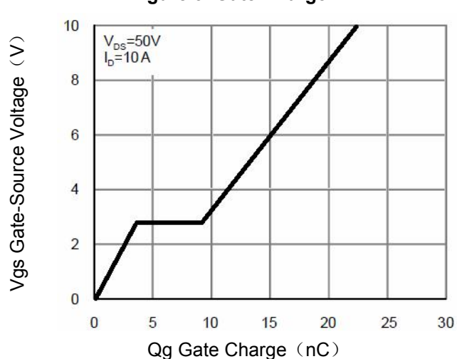
Figure 3. Gate Charge
