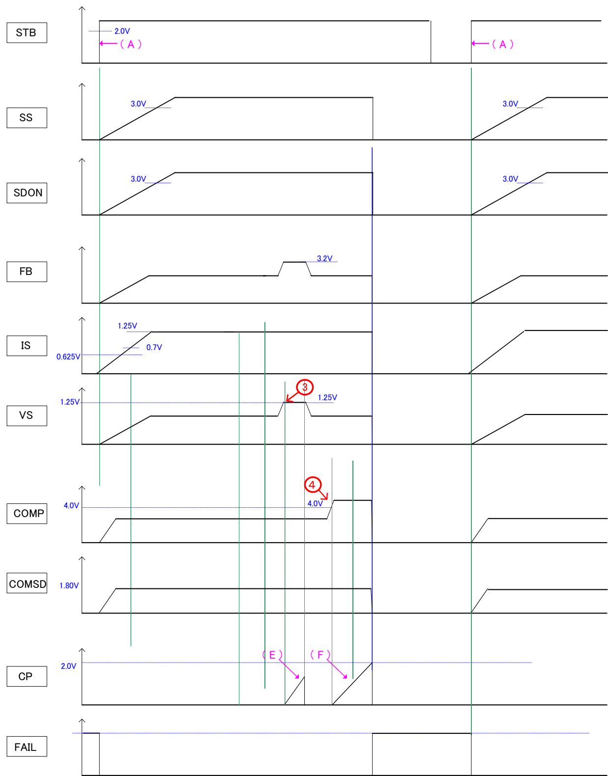
Figure. 26 Timing Chart 2
