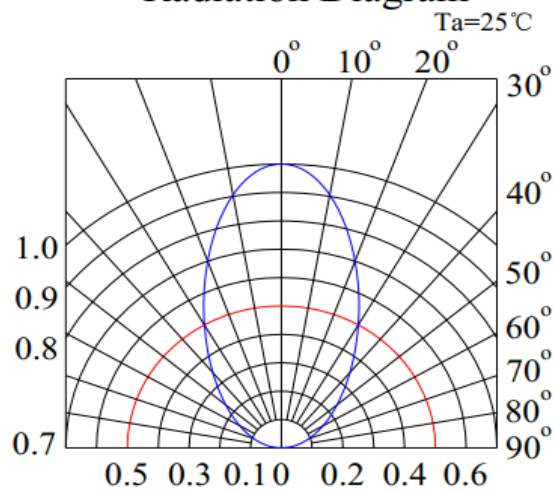
Radiation Diagram
