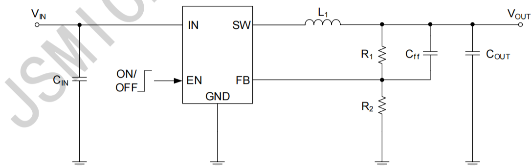
Basic Application Circuit
