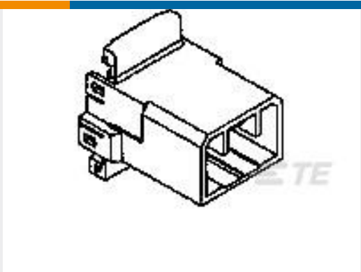
TE Part #174932-1 070 MLC W-W CAP HSG 10P
