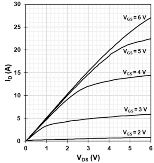
Figure 2 Typ. output characteristics
