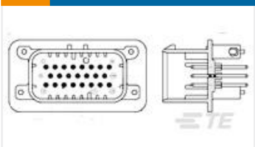
TE Part #1-776230-1 35POS,PIN DIA 1.3,HDR ASSY, 180DEG,COD 1
