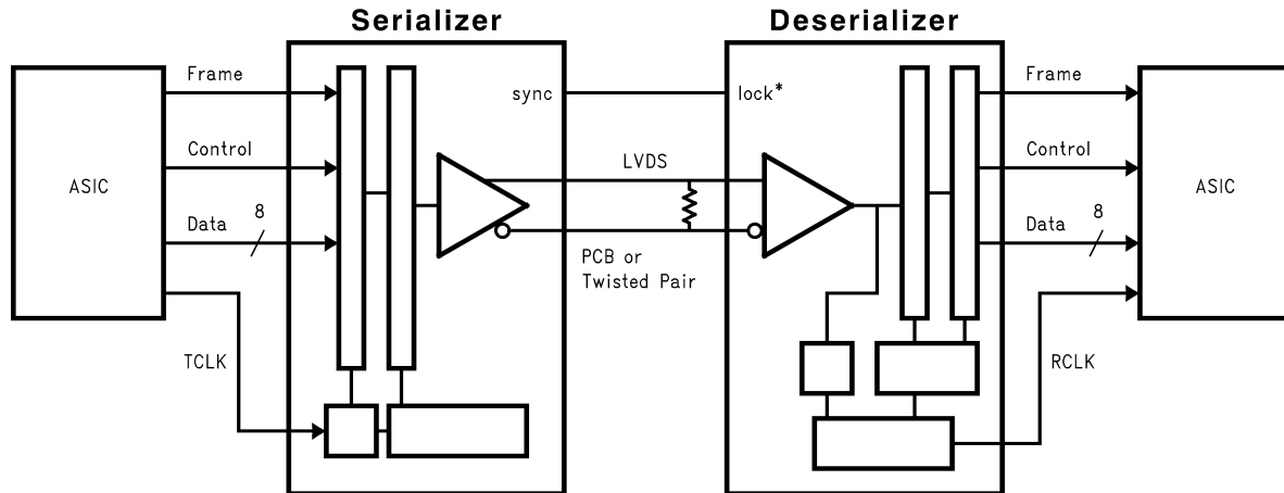
Figure 1. Application
