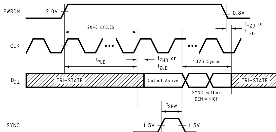
Figure 9. Serializer PLL Lock Time, SYNC Timing and PWRDN TRI-STATE Delays
