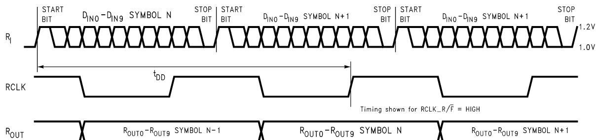
Figure 11. Deserializer Delay
