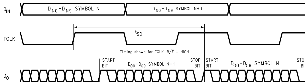
Figure 10. Serializer Delay
