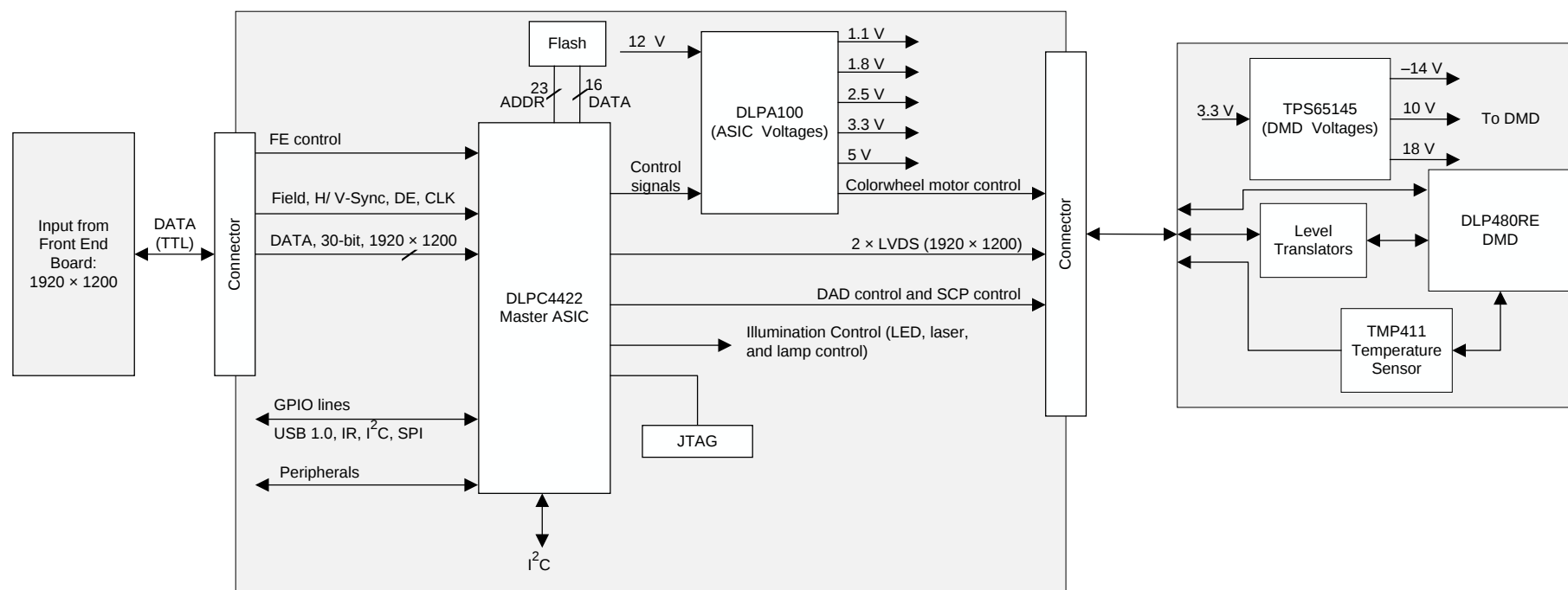
Figure 11. Typical WUXGA Application Diagram
